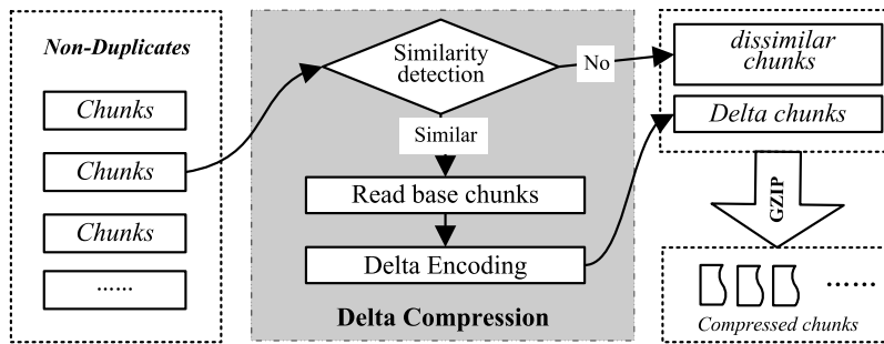
Fig. 6. The workflow of a post-deduplication data reduction (delta +GZ compression) system.
