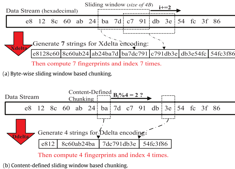
Fig. 1. A comparison between the classic Xdelta's byte-wise sliding window technique and Ddelta's deduplication-inspired content-defined sliding window technique for string matching in delta compression.
