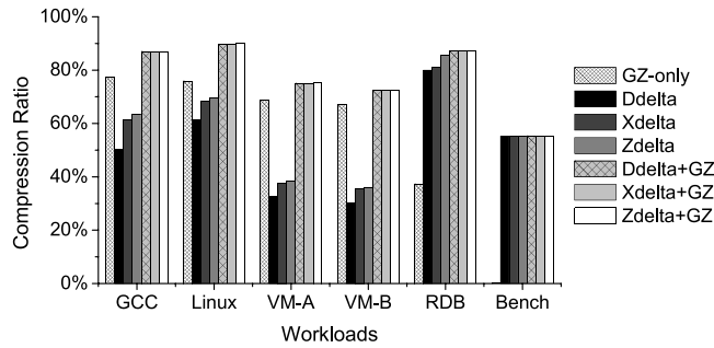
Fig. 9. Comparison in CR (compression ratio) among seven post-deduplication data reduction schemes.
