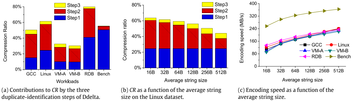
Fig. 7. A closer look at Ddelta, its three key steps for duplicate identification, i.e., Steps 1–3 of Fig. 3: (1) chunk-level greedily scanning for duplicates, (2) Gear-based duplicate-string identification, and (3) string-level greedily scanning for duplicates, and its sensitivity to the average string size for Gear-based chunking.
