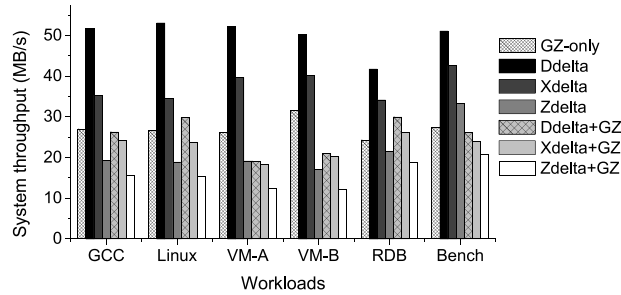
Fig. 10. Comparison in compressing throughput among seven post-deduplication data reduction schemes.
