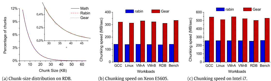
Fig. 5. Comparisons of chunk-size distribution and chunking speed between Rabin-based and Gear-based chunking approaches. Note that chunk-size distributions of other datasets are similar to and consistent with results of RDB in (a), and thus are omitted here.
