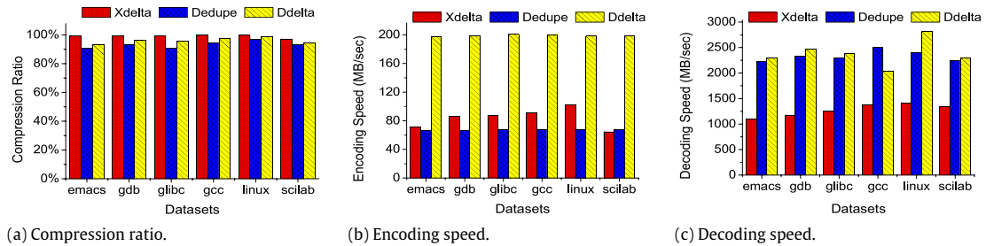
Fig. 12. Delta compression performance of updated tarred files by Xdelta, Deduplication, and Ddelta.
