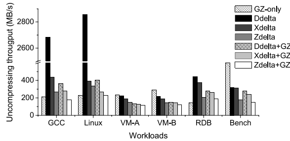
Fig. 11. Comparison in uncompressing throughput among seven post-deduplication data reduction schemes.
