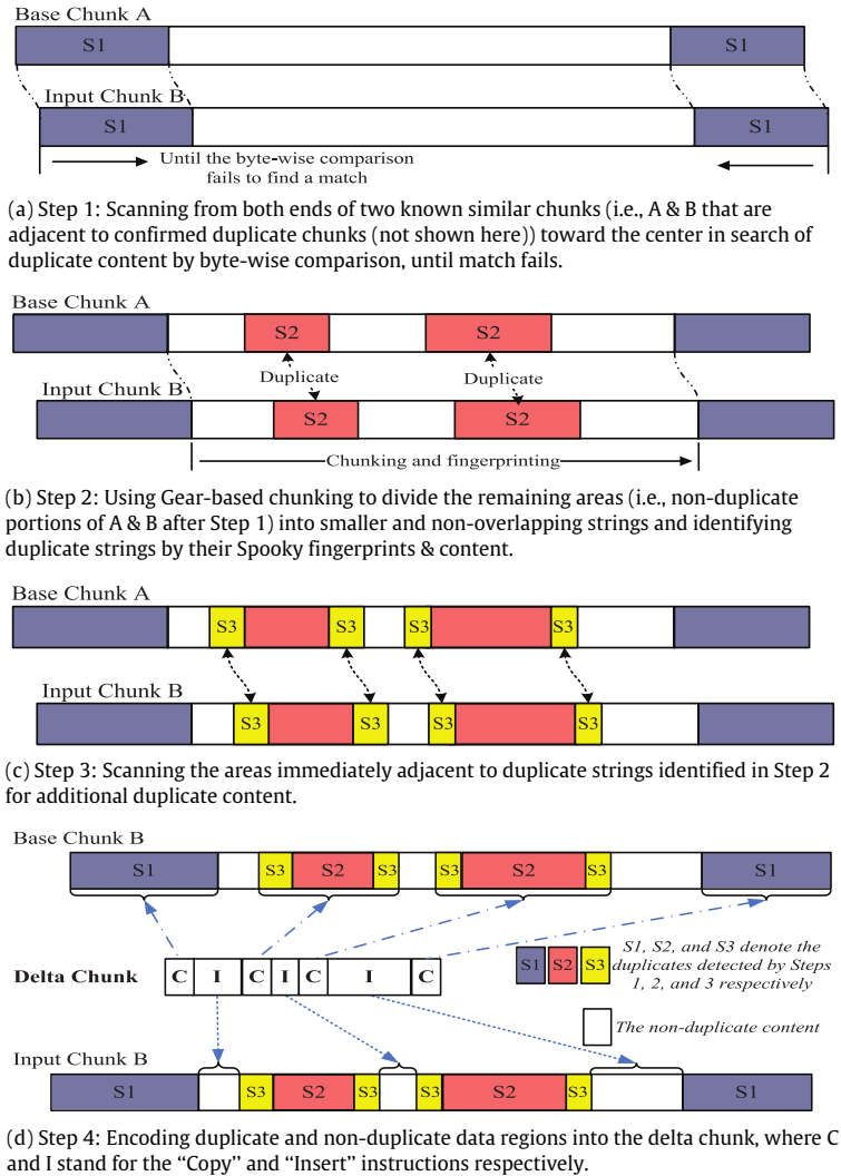
Fig. 3. The workflow of the Ddelta approach.
