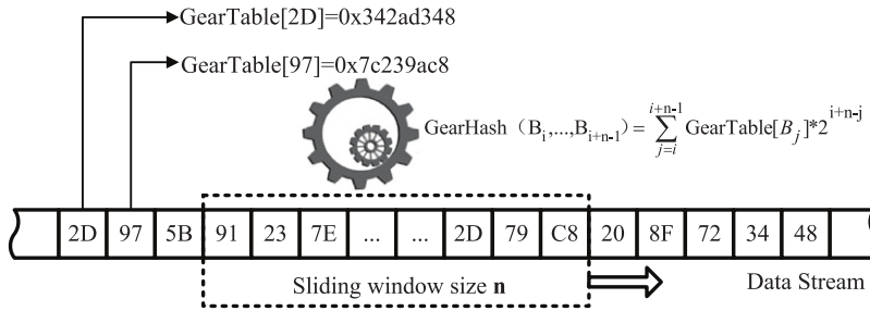
Fig. 2. Gear-based fast chunking.
