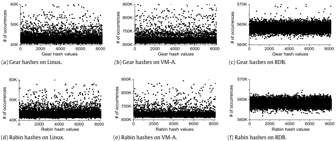
Fig. 4. A comparison of hash distribution between the Rabin-based and Gear-based chunking schemes. Here the X axis shows the masked hash values, that is, the 13 most/least significant bits of the Gear/Rabin hash values for CDC with an average chunk size of 8 KB in a deduplication system. The Y axis indicates the total number of occurrences of hashing that result in the same masked hash value.
